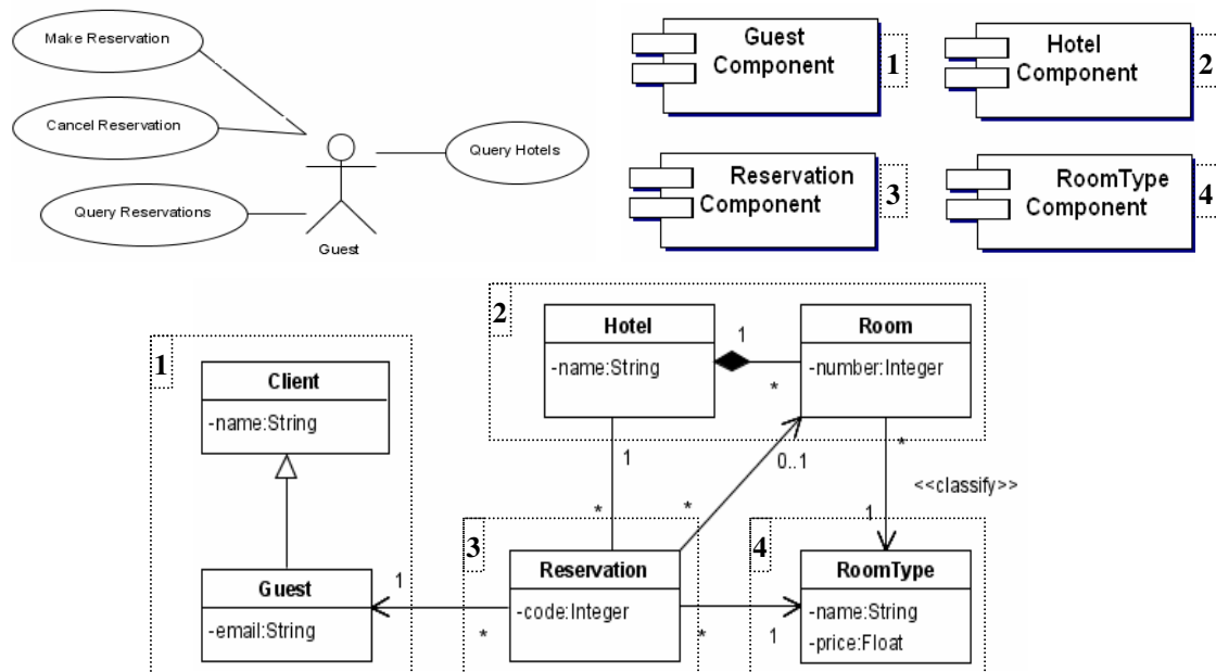
Figure 4. Use case, class, and component diagrams used in the example
