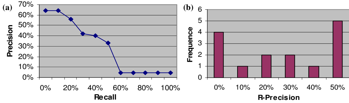
Figure 7. (a) Precision x recall curve and (b) R-Precision histogram
